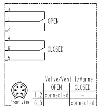
Wiring diagram
