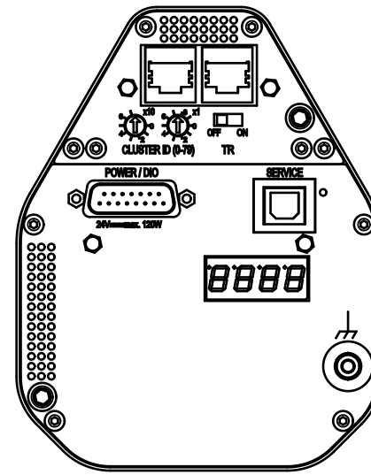
Valve Cluster Slave (without interface)
