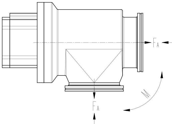
Angle valve
